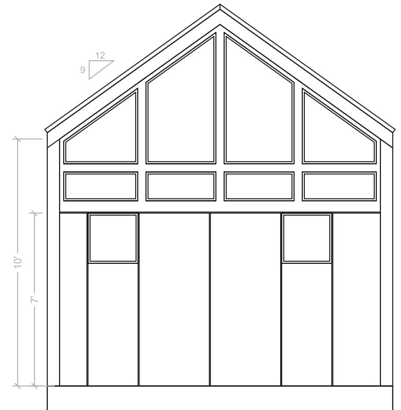
Maurice 20x14 Rear Elevation (Bath and Kitchen Configuration)
