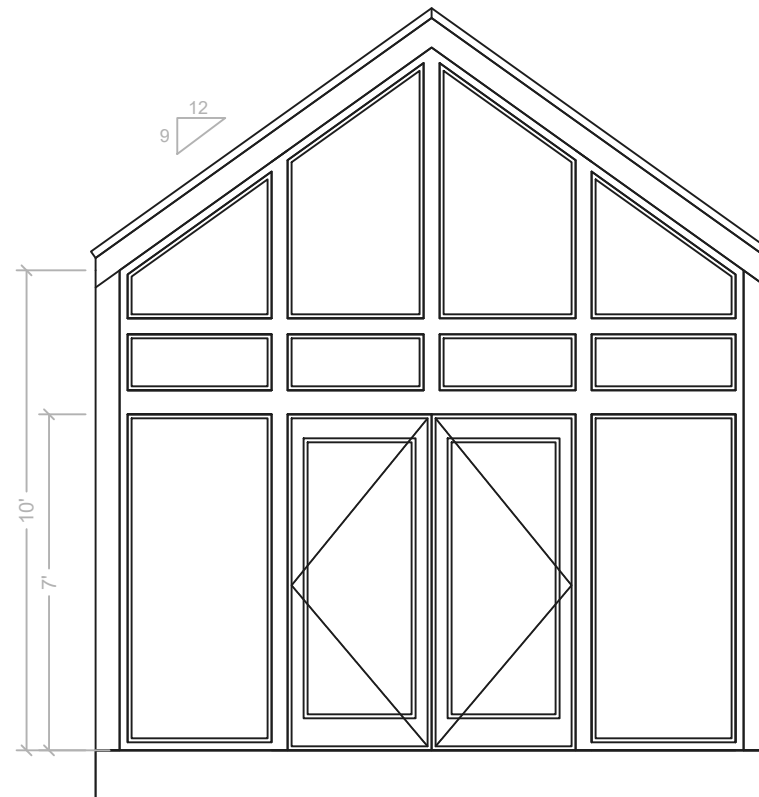
Maurice 20x14 Front Elevation
