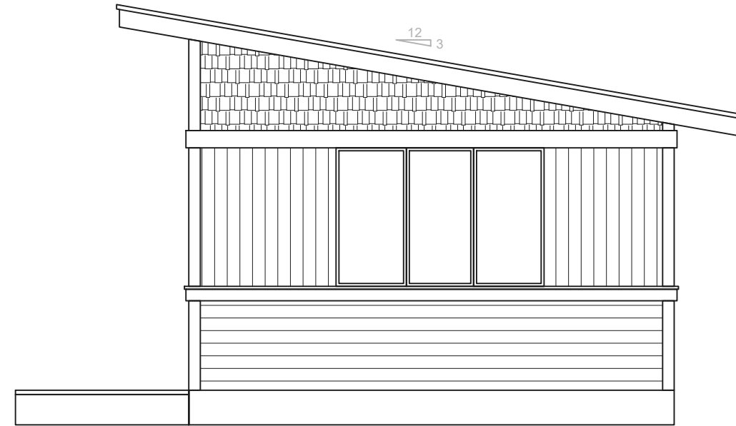
Moderno 14x14 Side Elevation
