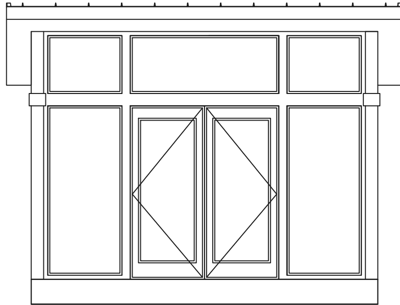
Moderno 14x14 Front Elevation
