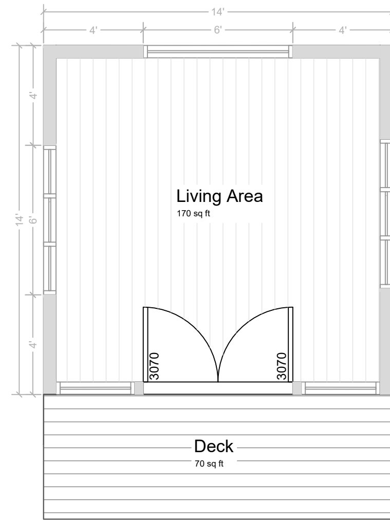
Moderno 14x14 Open Floor Plan
