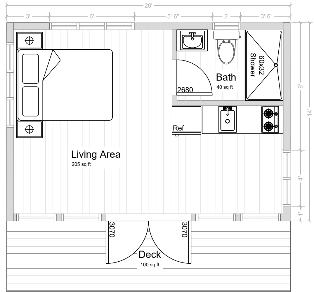
Moderno 20x14 Floor Plan
