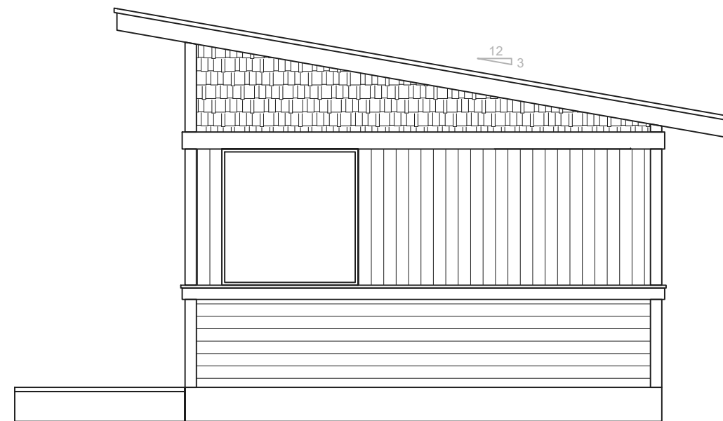
Moderno 20x14 Side Elevation
