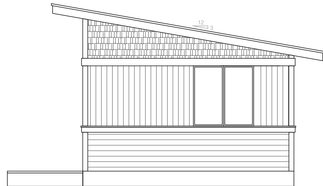
Moderno 28x14 Side Elevation
