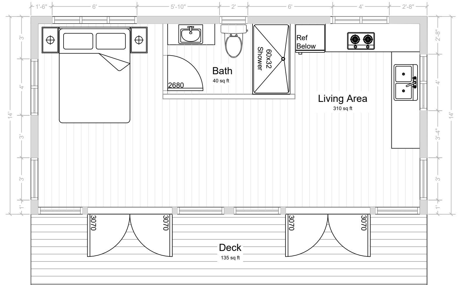
Moderno 28x14 Floor Plan
