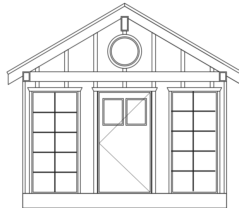
Moose 20x14 Front Elevation
