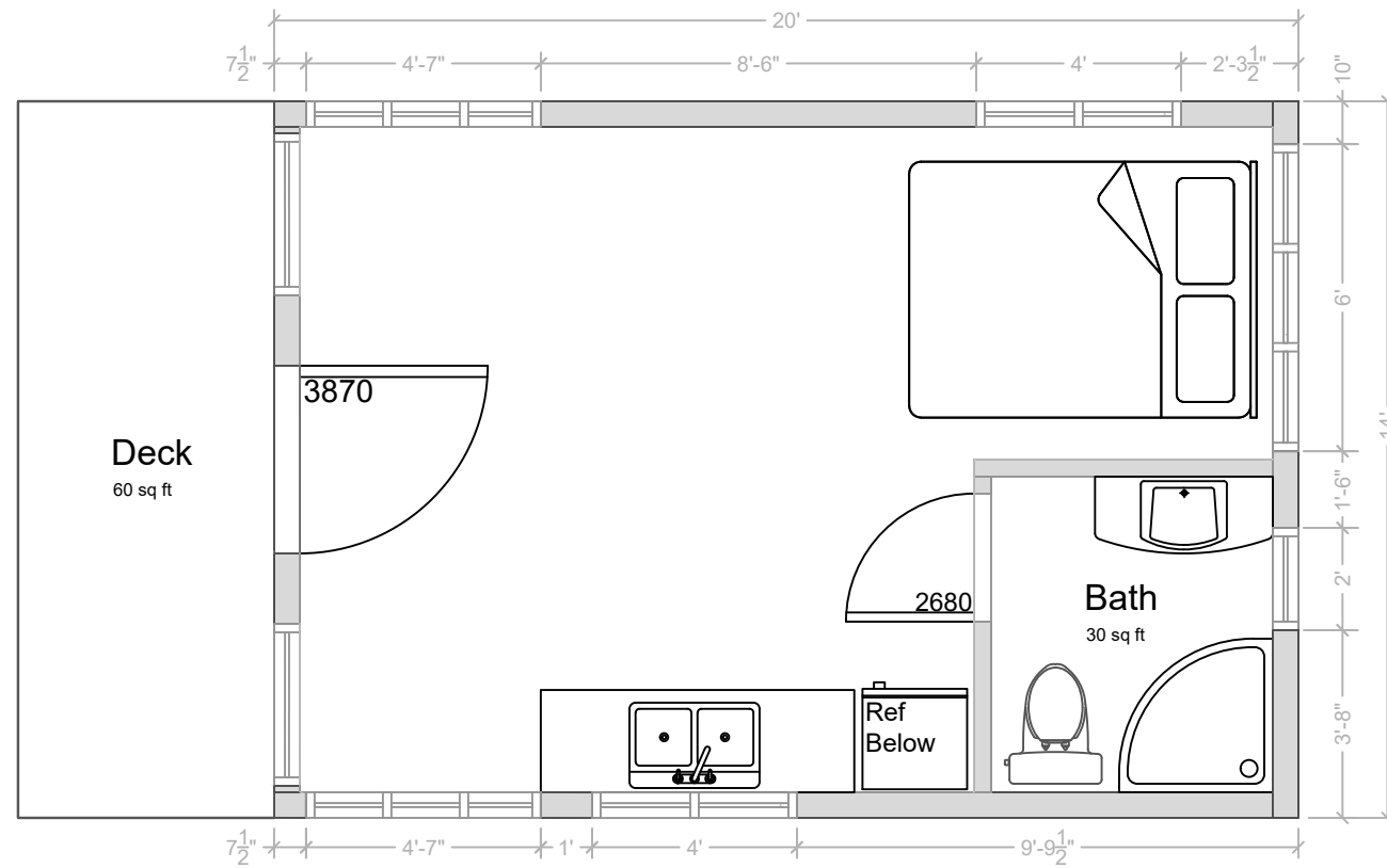
Moose 20x14 with Kitchen
