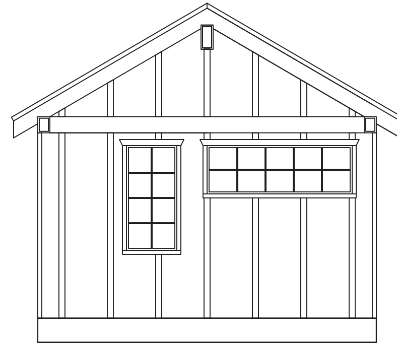
Moose 20x14 Rear Elevation
