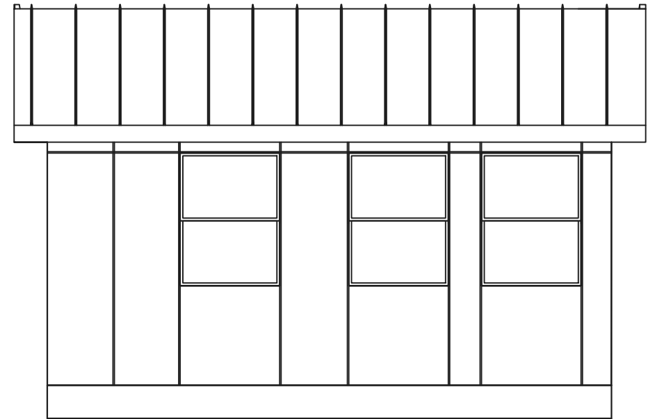
CeVonne 14x14 Back Elevation
