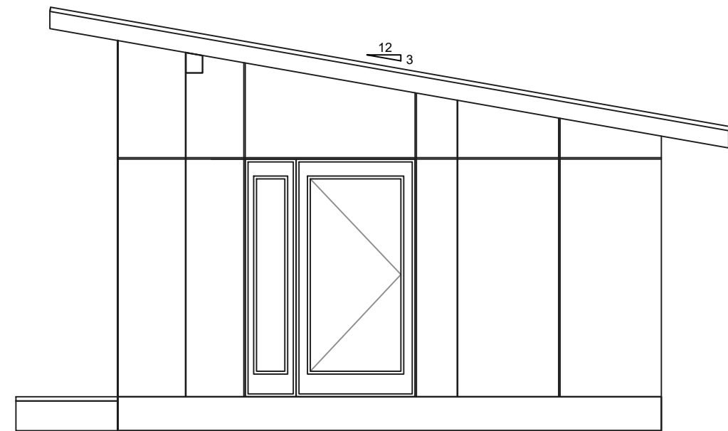
CeVonne 14x14 Side Elevation
