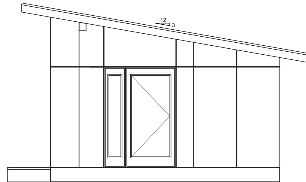
CeVonne 20x14 Side Elevation
