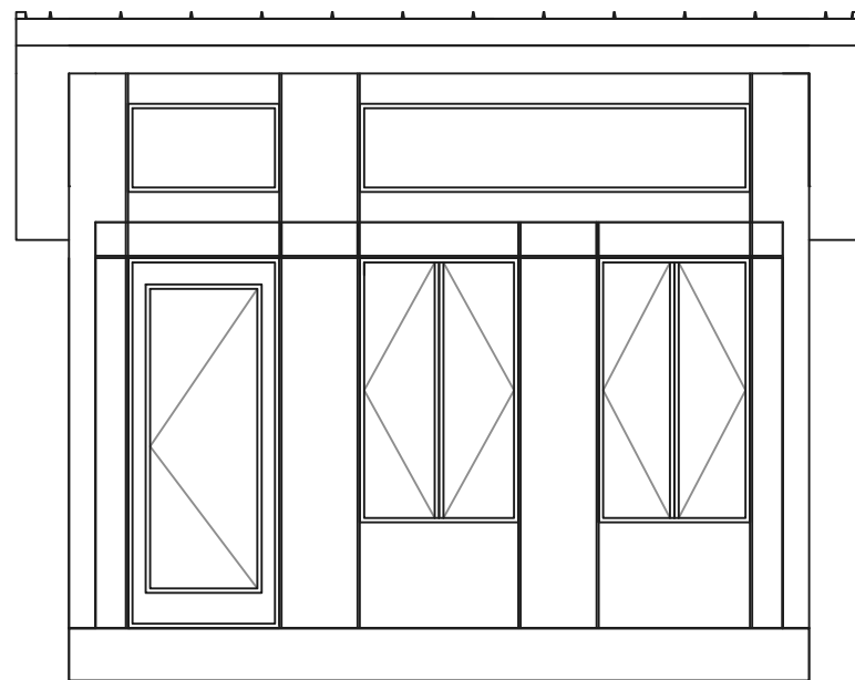
Point Grace 14x14 Front Elevation
