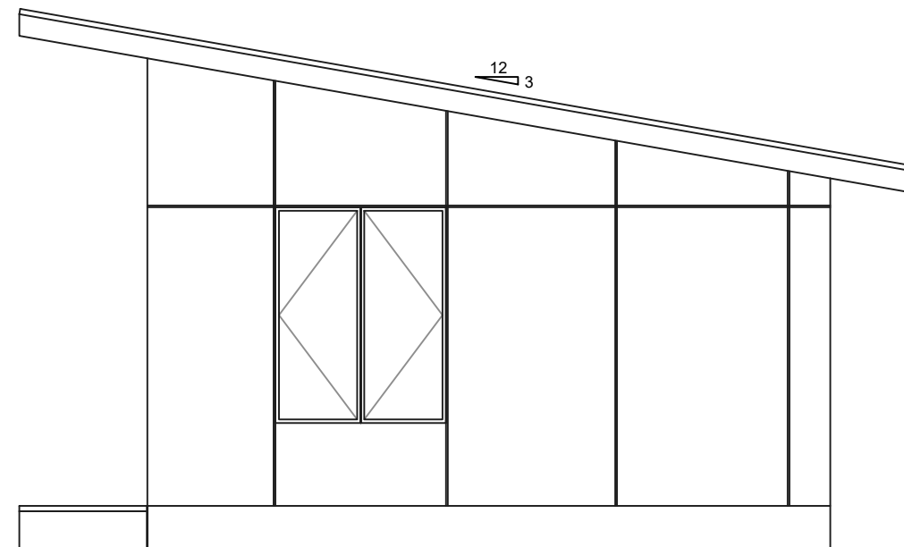
Point Grace 20x14 Side Elevation
