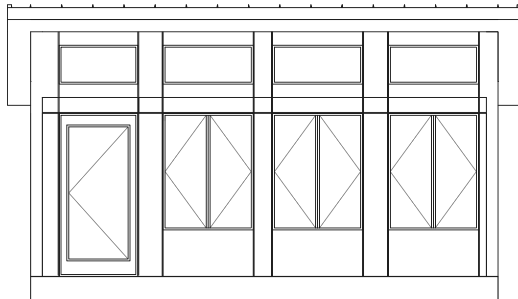
Point Grace 20x14 Front Elevation
