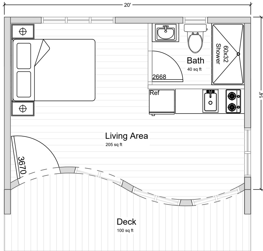
Point Grace 20x14
