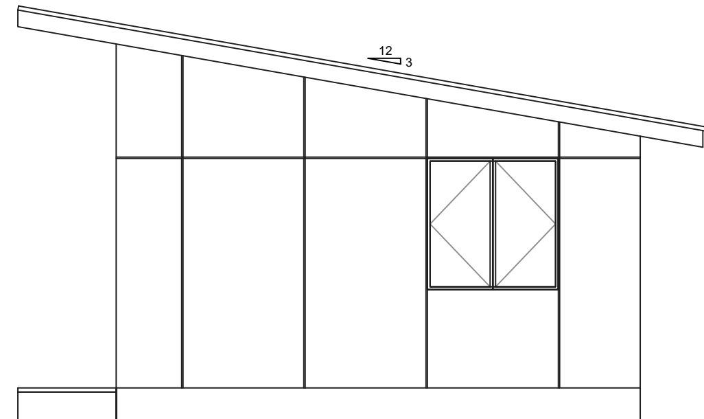
Point Grace 28x14 Side Elevation
